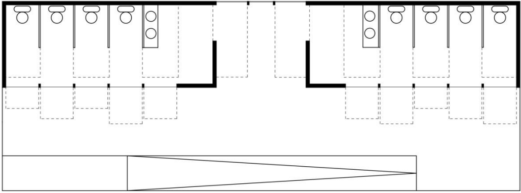
Plan 1cm:1m
